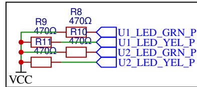
Ethernet LED Connections
