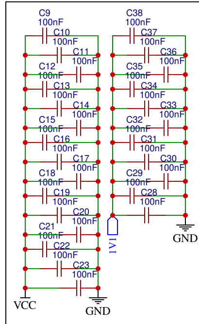
Decoupling Capacitors
