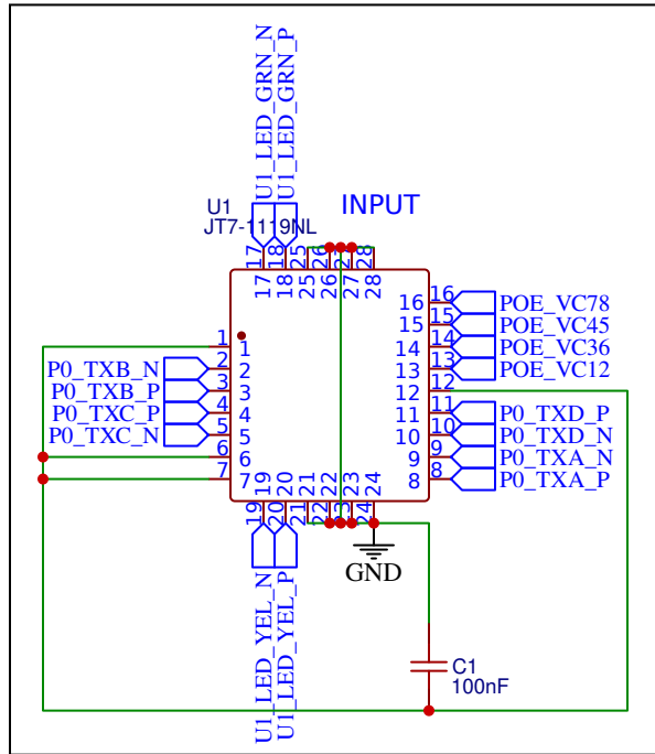
Ethernet Port (Input)
